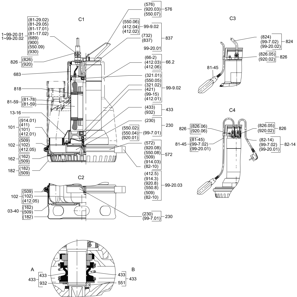
III. 15: Plan d'ensemble AmaDrainer 4../10, 4../35, 5../10K
