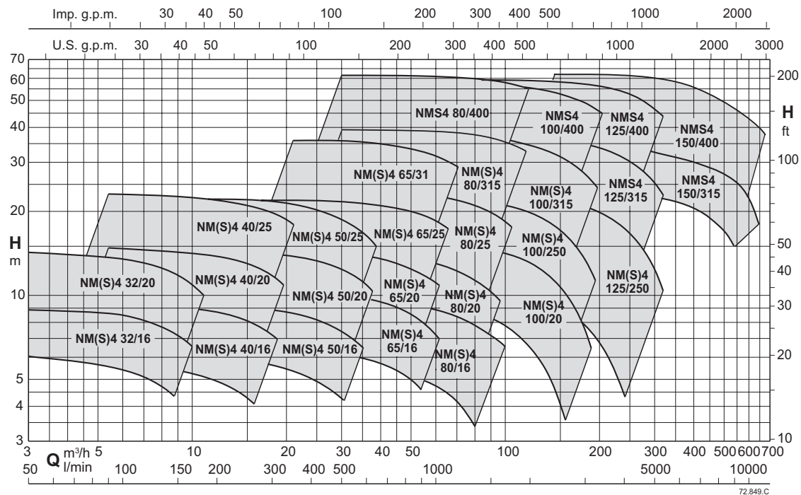
Performances n ≈ 1450 1/mi
